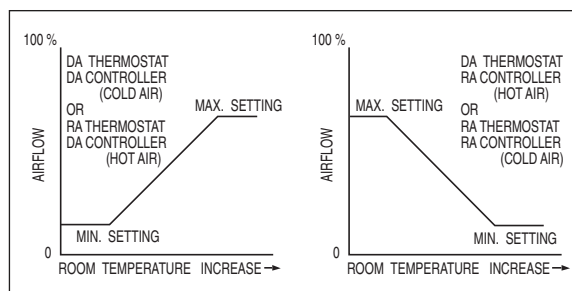
Figure 23. Thermostat/Controller Interaction
