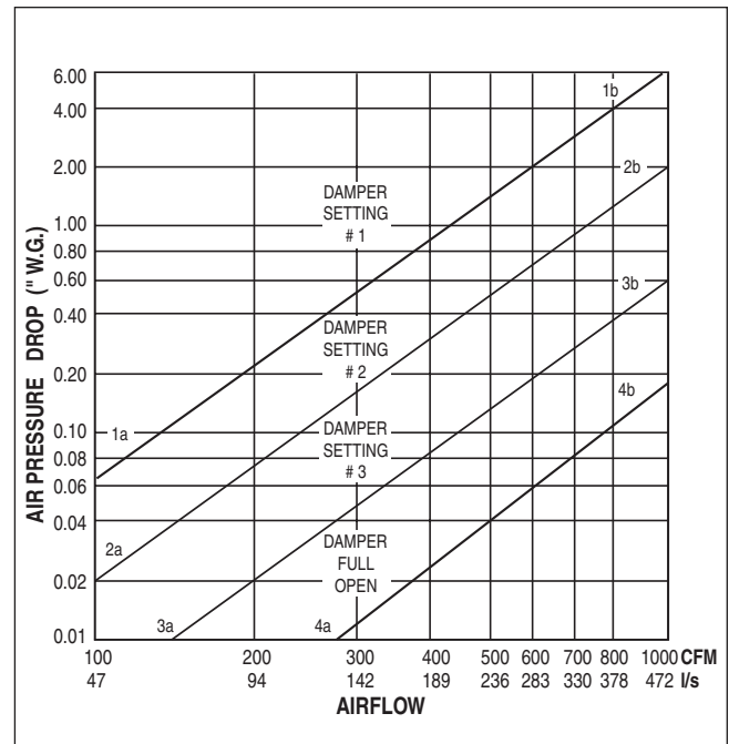
Figure 13a. Pressure Dependent terminal damper characteristics.
