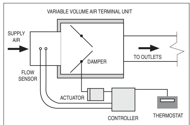
Figure 14b. Pressure Independent terminal controls.
