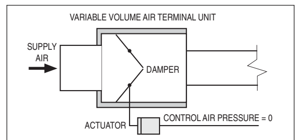
Figure 21. Normally Closed Damper
