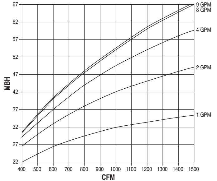
2 Row (multi-circuit)
