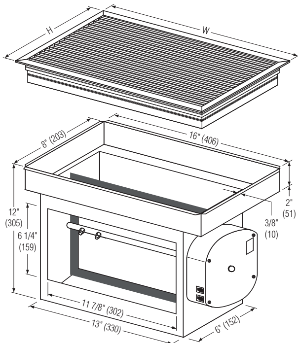
Model NLD-VH - VAV - Heating Only - Non-ducted
