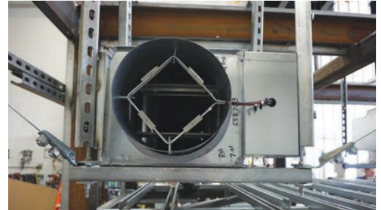
Single Duct Terminal Unit in Trapeze
