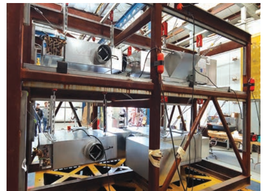
Fan Powered Terminal Units Shake Table Test
