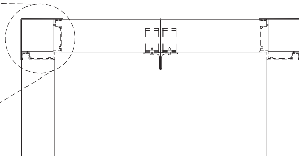
BOX (POST) CORNER DETAIL
