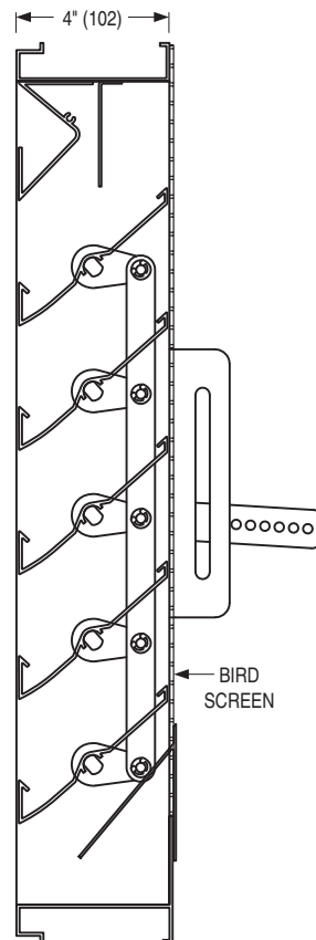
OPT. FLANGED FRAME (FL15 STD.)
