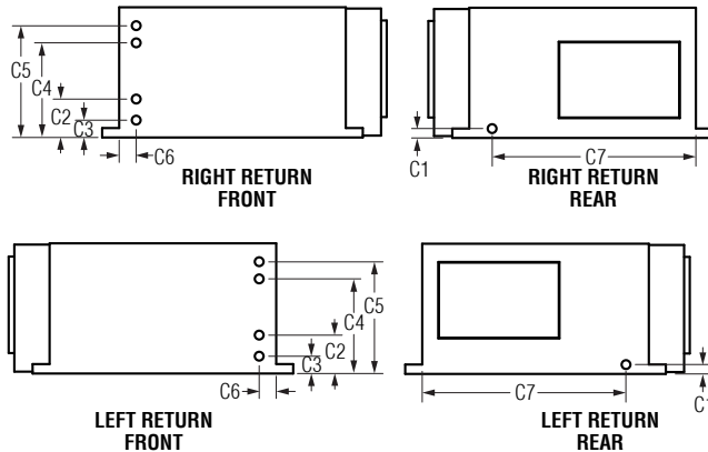
Dimensions Data - Coil Connections
