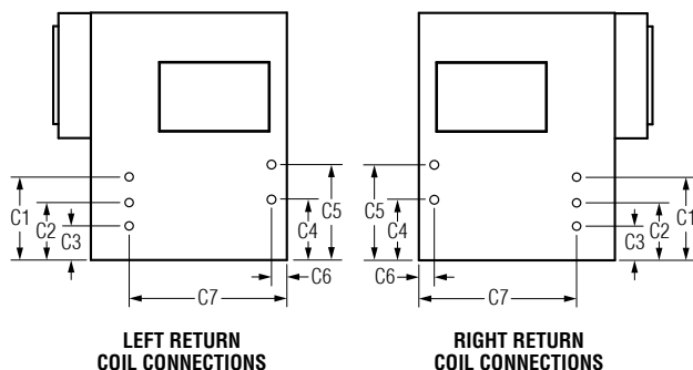
Dimensions Data - Coil Connections
