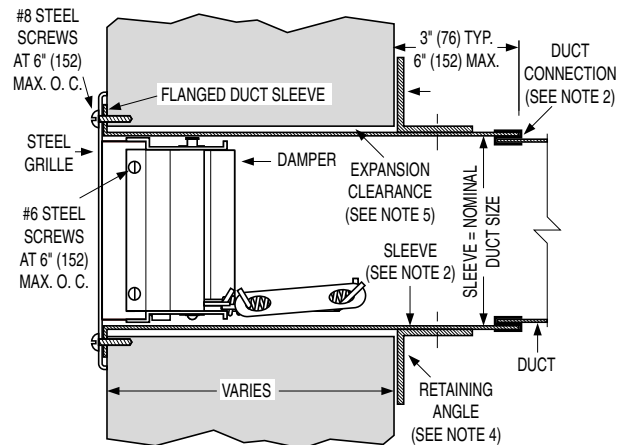
SIDEWALL INSTALLATION WITH GRILLE
