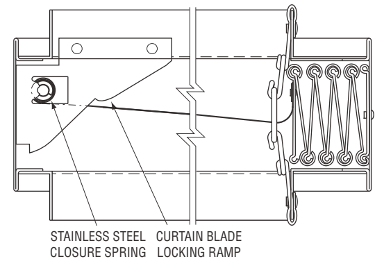
HORIZONTAL MOUNT
