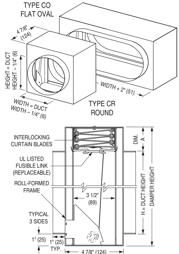
MODEL D0530SS – CO / CR – VERTICAL MOUNT
