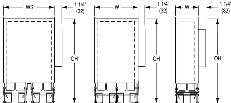
Frame / Border GGS Straddle Mount
