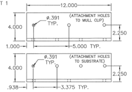
(158) 4x4x3/8" ALUMINUM MOUNTING ANGLE @ MULLS
