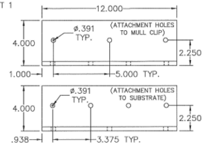
158 4x4x3/8" ALUMINUM MOUNTING ANGLE @ MULLS
