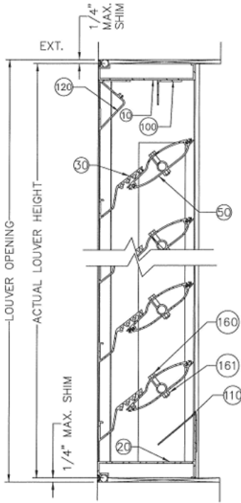
A 3 VERTICAL SECTION DETAIL
