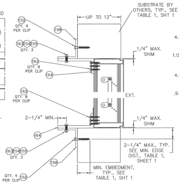
3xXx1/2" STEEL MULL CLIP HEAD/SILL OPTIONAL ATTACHMENT TO UP TO 12" WALL WITH 4x4x3/8" ALUMINUM MOUNTING ANGLE
