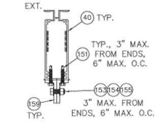
VERTICAL MULLION ASSEMBLY
