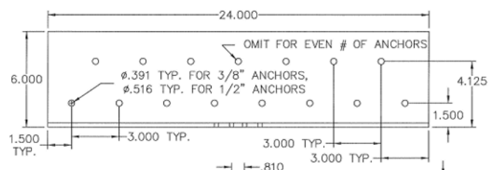
3x6x1/4" ALUMINUM MULL CLIP HEAD/SILL ATTACHMENT TO SUBSTRATE
