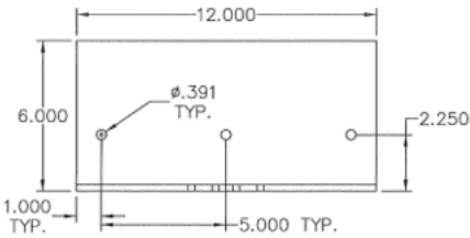
155 MULL ATTACHMENT WITH 3x6x1/4" MOUNTING CLIP AND 4x4x3/8" MOUNTING ANGLE
