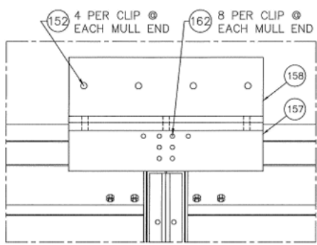
(A) (6) MULL ATTACHMENT WITH 3xXx1/2" STEEL MOUNTING CLIP AND 4x4x3/8" MOUNTING ANGLE
