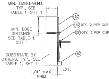
A 3x6x1/4" ALUM. JAMB CLIP ATTACHMENT TO SUBSTRATE
