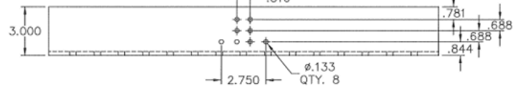
157 3x6x1/4" ALUMINUM MULL CLIP FOR ATTACHMENT TO SUBSTRATE
