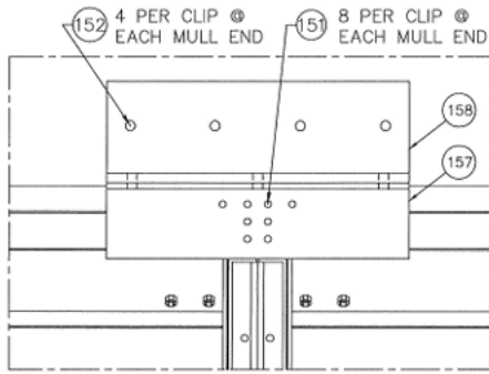
155 MULL ATTACHMENT WITH 3x6x1/4" MOUNTING CLIP AND 4x4x3/8" MOUNTING ANGLE
