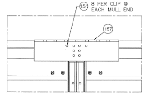
Ⓐ 3x6x1/4" ATTACHMENT TO LOUVER WITH MULL CLIP DIRECT TO SUBSTRATE
