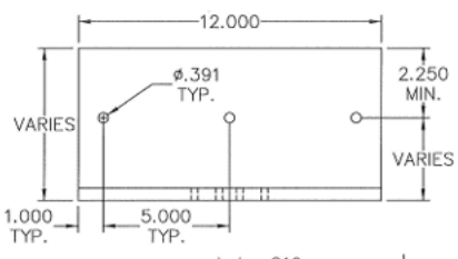
(A) (6) MULL ATTACHMENT WITH 3xXx1/2" STEEL MOUNTING CLIP AND 4x4x3/8" MOUNTING ANGLE
