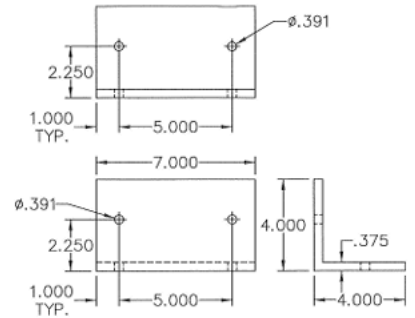
158 4x4x3/8" ALUM. MOUNTING ANGLE @ JAMBS
