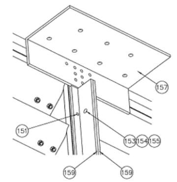
MULLION VIEW FROM INTERIOR
