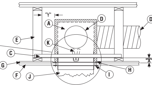
END VIEW WITH DUCT (0757D)
