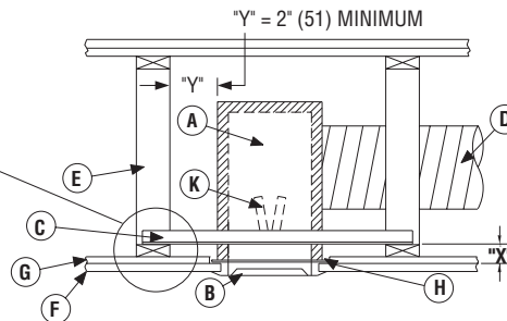
END VIEW WITH GRILLE (0757)
