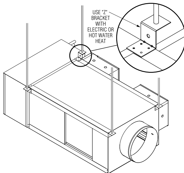
Figure 2: Fan Powered Terminal Unit Support Using Hanger Brackets and Rods (Models 35SWST and 35SW illustrated).
