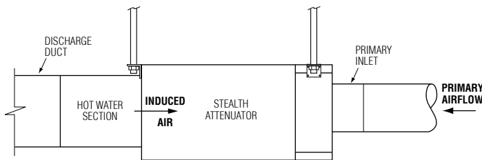
Figure 1: Fan Powered Terminal Unit Support Using Hanger Straps (Model 35SE illustrated).
