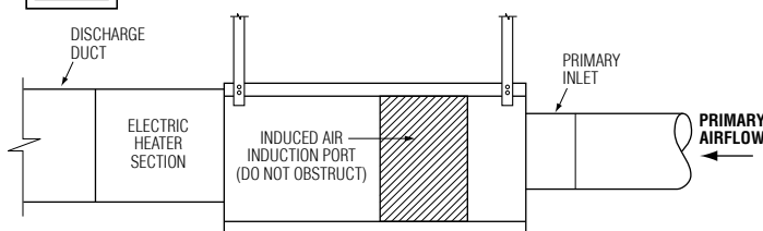
Figure 1: Fan Powered Terminal Unit Support Using Hanger Straps (Model 35SE illustrated).
