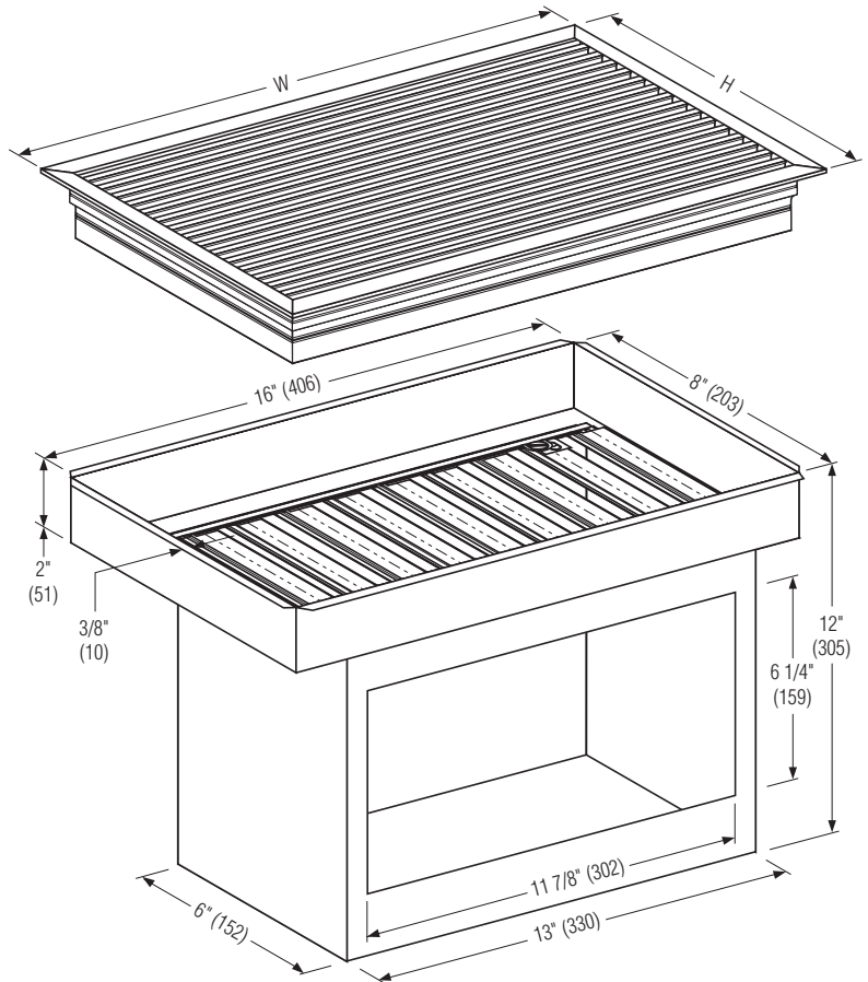
FLOOR OPENING = 16 1/4" x 8 1/4" (413 x 210) W = 17 5/8" (448) FOR FRAME F OR 17 1/8" (435) FOR FRAME H H = 9 5/8" (244) FOR FRAME F OR 9 1/8" (232) FOR FRAME H
