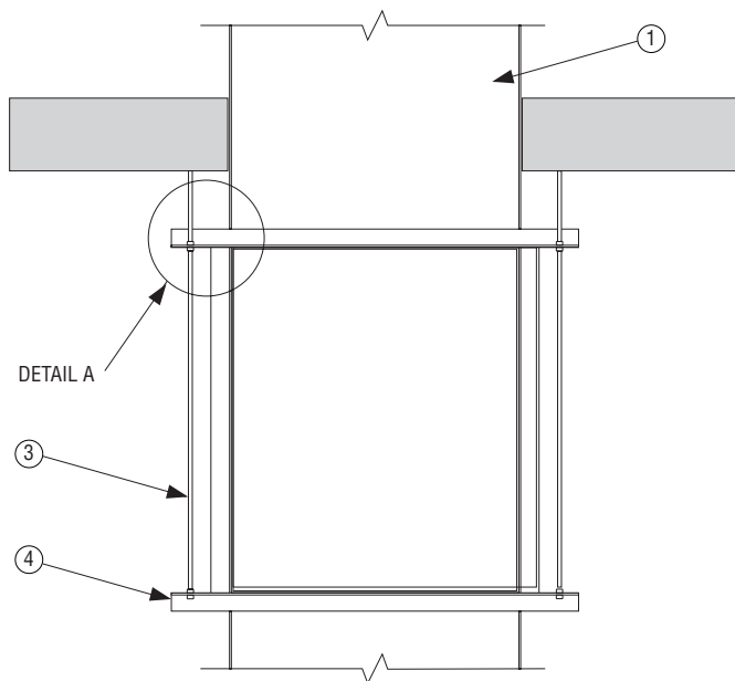
END VIEW
