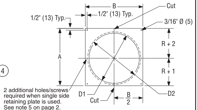
Damper and Retaining Plates Detail
