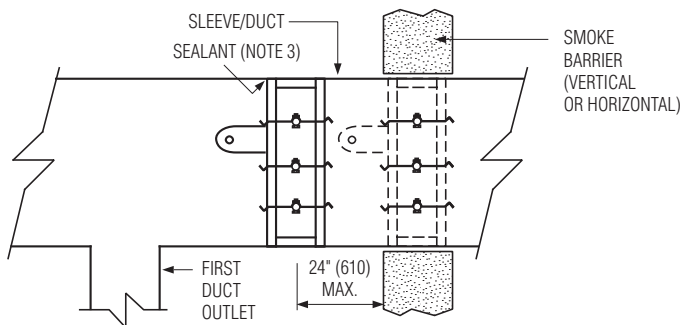
Model Series: 1210, 1260, 1280 Multi-Blade Damper
