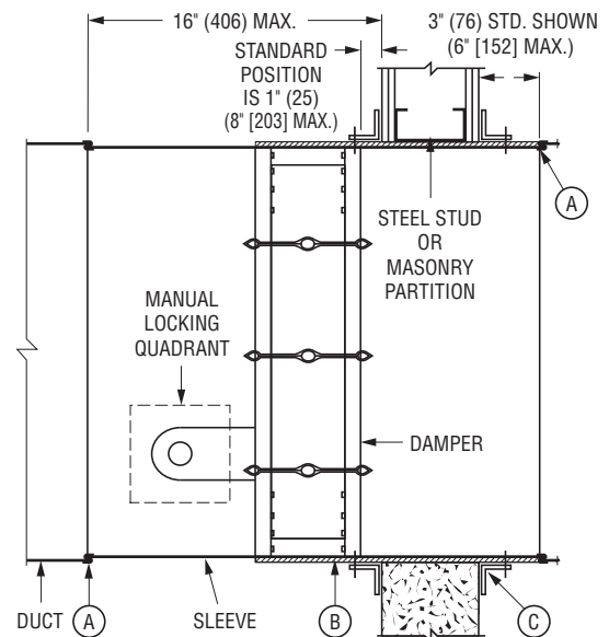
VERTICAL INSTALLATION
