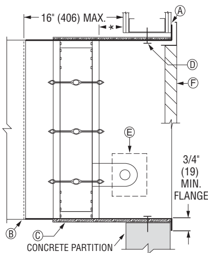
VERTICAL MOUNT
