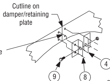
Splice Detail
