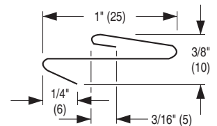
Std. 26 Ga. Boot Rail
