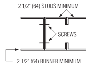
Framing Detail Section A-A
