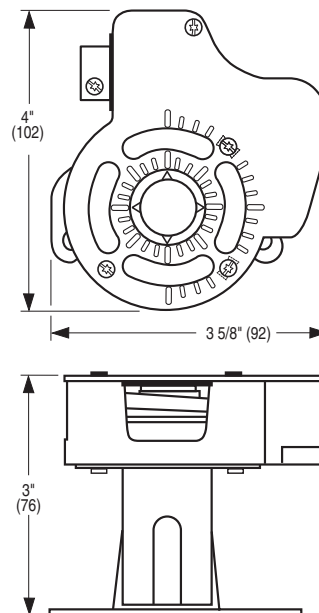
Figure 2. Dimensional detail
