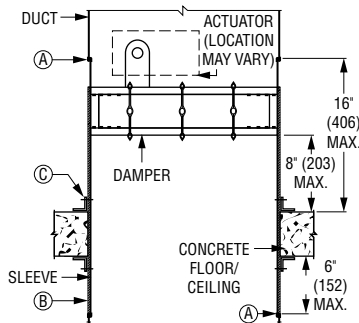
ABOVE FLOOR INSTALLATION
