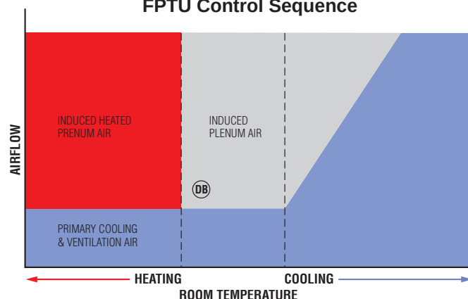
Traditional Constant Volume FPTU Control Sequence
