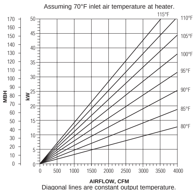
Heater Selection Chart
