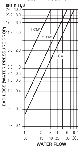
Water Pressure Drop
