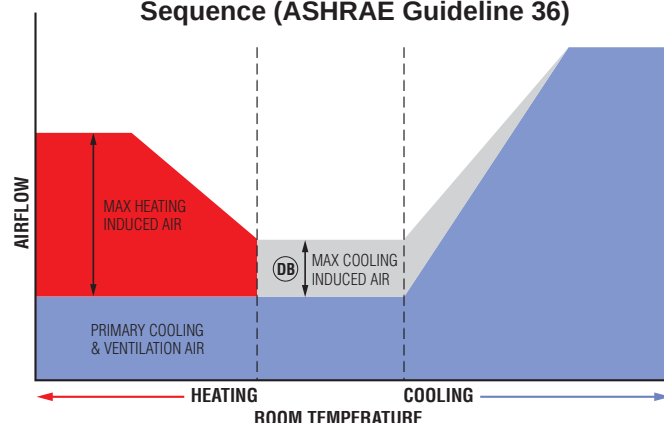
Advanced Variable Volume FPTU Control Sequence (ASHRAE Guideline 36)
