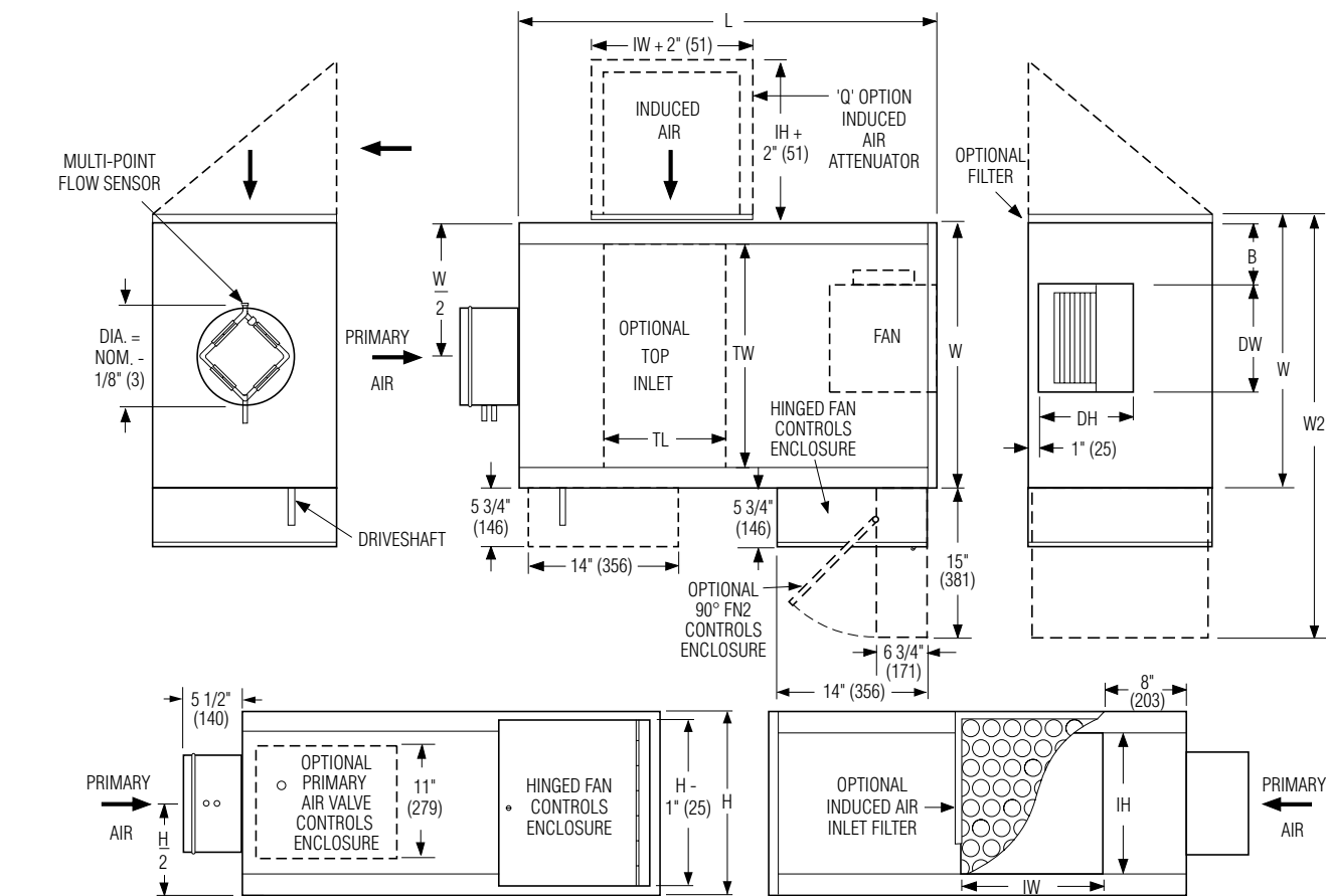
Dimensional Data
