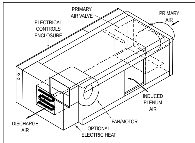
Figure 1. Series Fan Terminal
