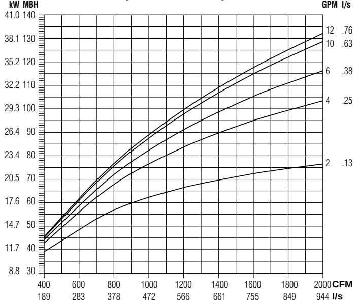
4 Row (multi-circuit)
