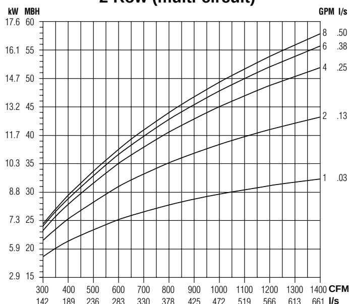
2 Row (multi-circuit)
