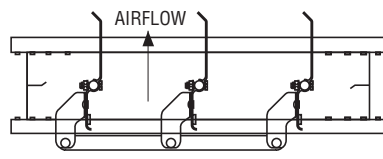
Horizontal Mount – Airflow up (Option HMU)
