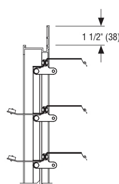
Front Flange (on discharge side) (Option FF)
