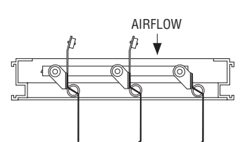
Horizontal Mount – Airflow down (Option HMD) (Available on all frame styles)
