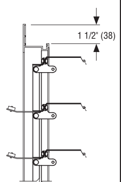
Rear Flange (on intake side) (Option FR)
