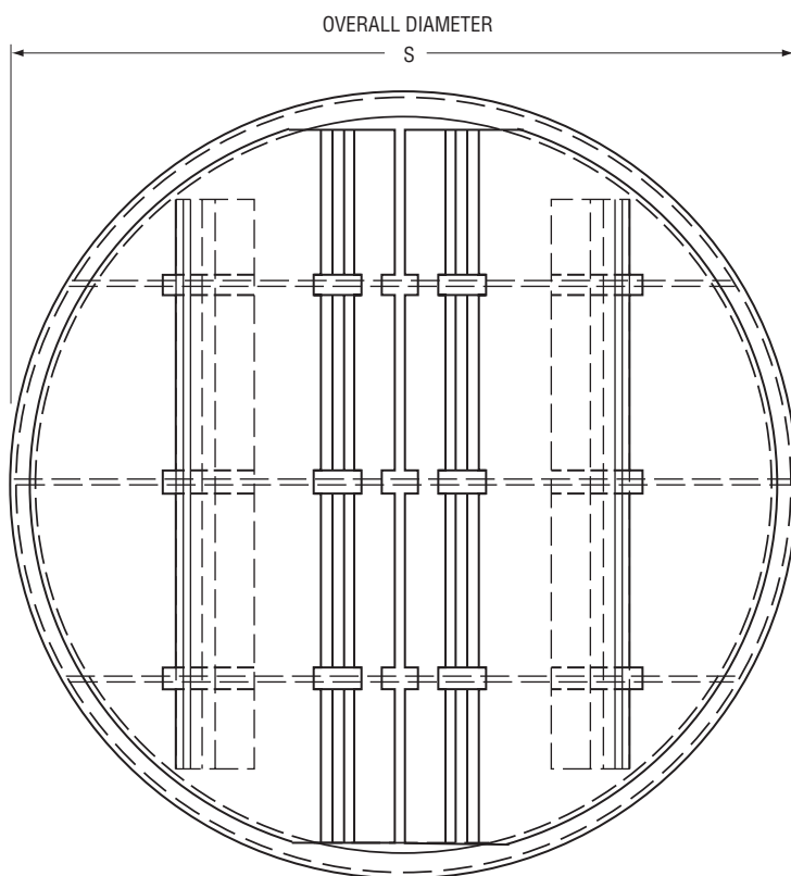
TOP VIEW VALVES CLOSED
