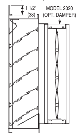
OPT. FLANGED FRAME (FL15 STD.)
