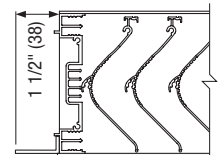
OPT. FLANGED FRAME (FL15 STD.)
