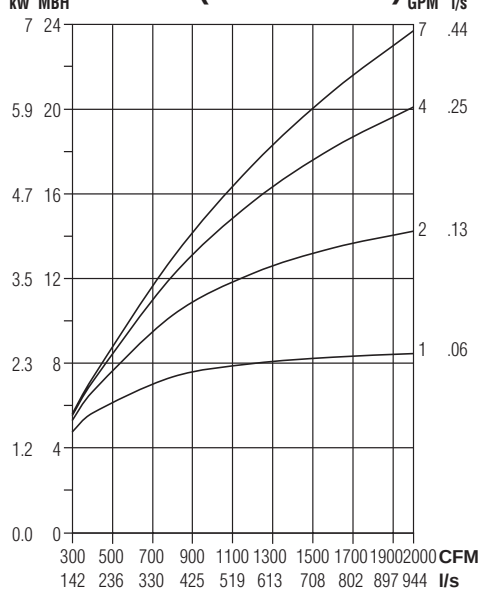
4 Row (multi-circuit)
