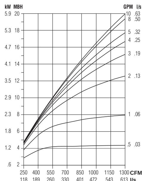
6 Row (multi-circuit)
