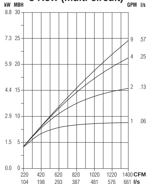
8 Row (multi-circuit)
