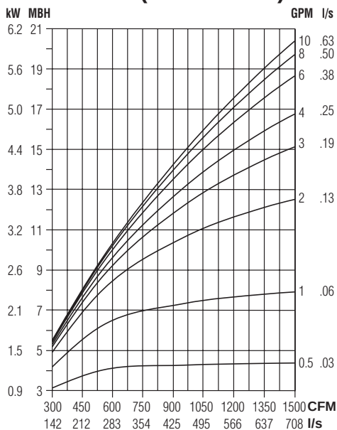
4 Row (multi-circuit)
