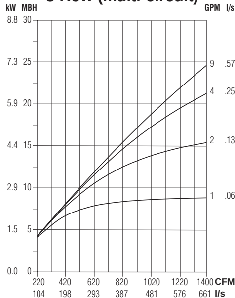
8 Row (multi-circuit)
