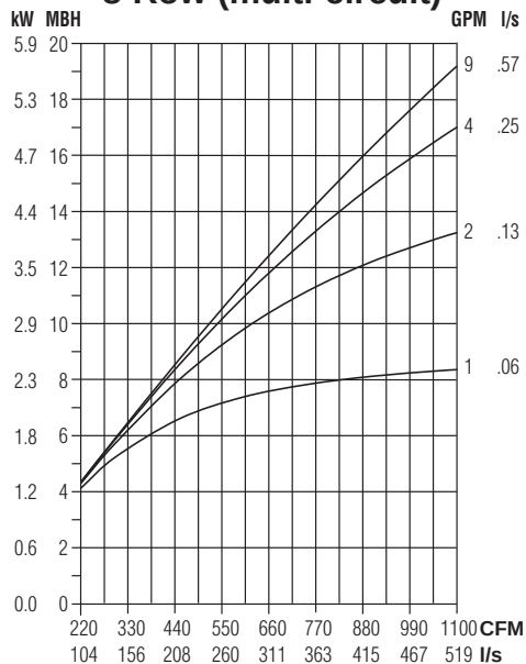
8 Row (multi-circuit)
