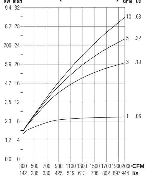
6 Row (multi-circuit)
