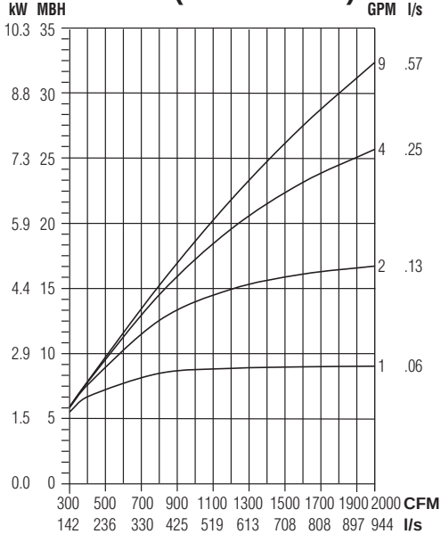
8 Row (multi-circuit)
