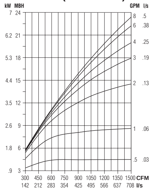
6 Row (multi-circuit)
