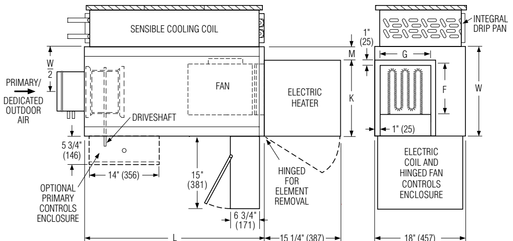
Dimensional Data
