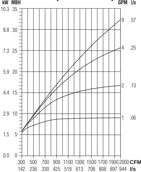
8 Row (multi-circuit)
