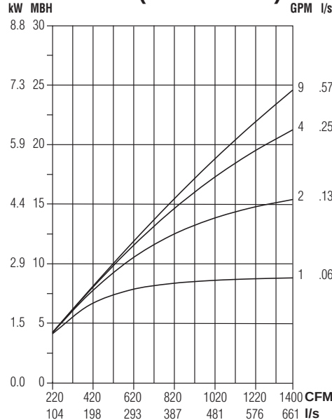
8 Row (multi-circuit)
