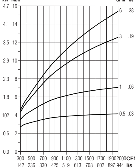
2 Row (multi-circuit)
