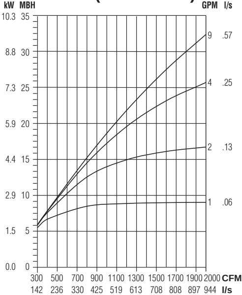
8 Row (multi-circuit)
