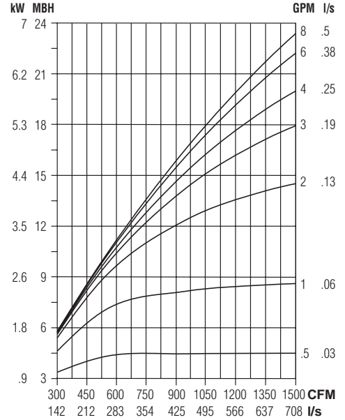
6 Row (multi-circuit)
