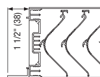
OPT. FLANGED FRAME (FL15 STD.)
