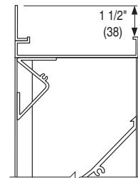
OPT. FLANGED FRAME (FL15 STD.)
