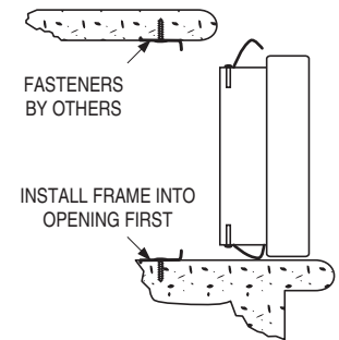
RISER MOUNT DETAIL
