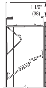
OPT. FLANGED FRAME (FL15 STD.)
